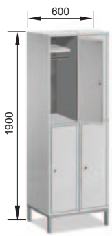
RSK2 2/300
