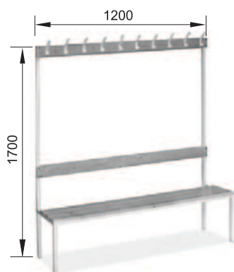
1IPN/1200
