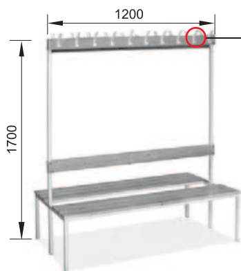
2IPN/1200
