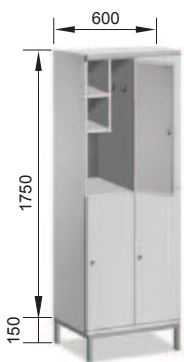
SKK22/300+TR
