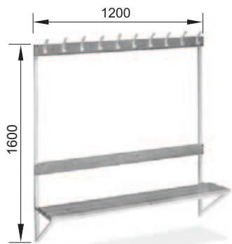
1IPN/1200
