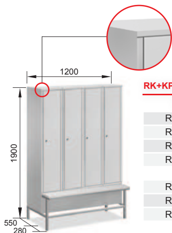
RK4/300+KP
