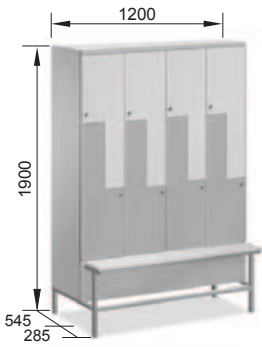
ZGK4/300+KP
